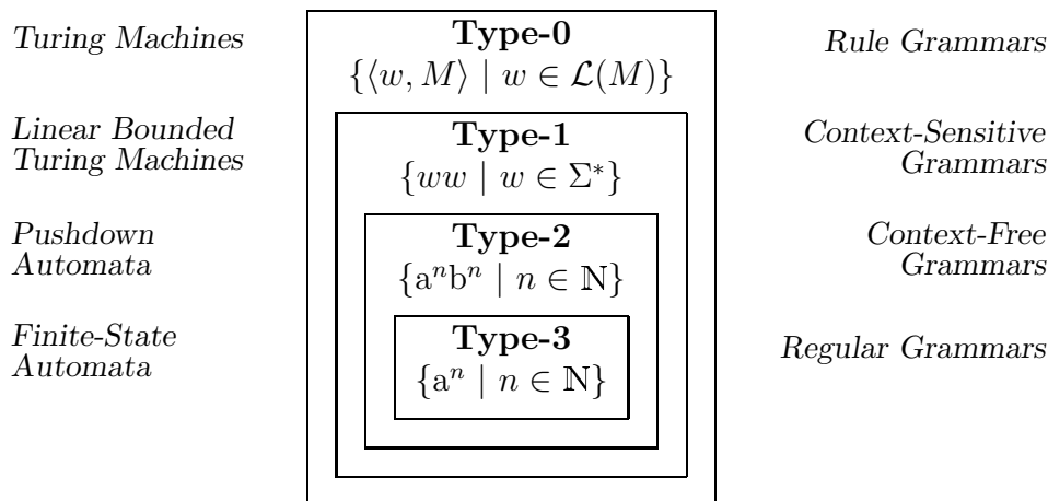
Figure 1: The Chomsky hierarchy of weak generative capacity
